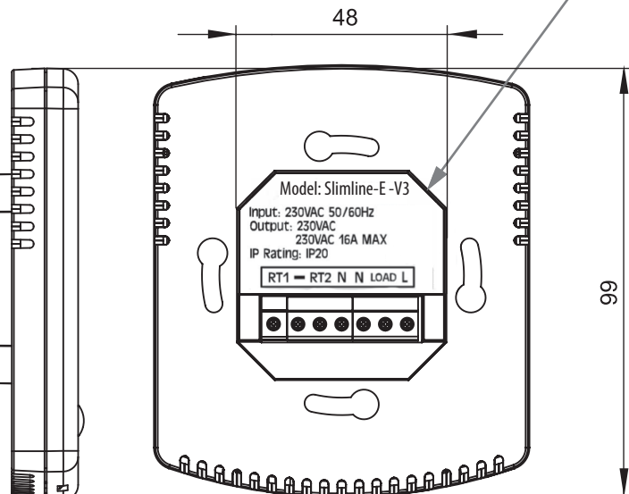
Wiring Detail
